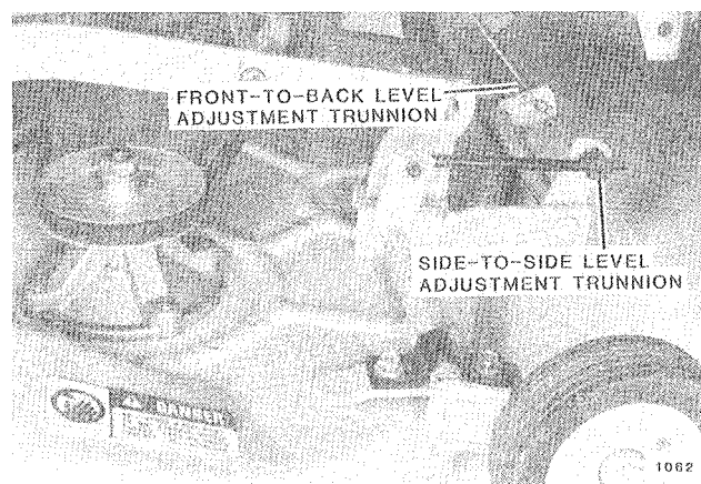
FIG. 15. 37 inch (94 cm) Mower Side-to-Side Leveling
