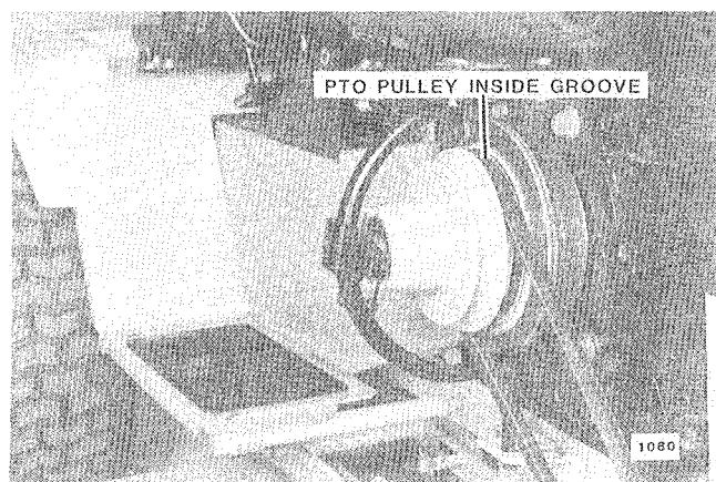
FIG. 12. 36, 42, 48 Inch Mower PTO Pulley
