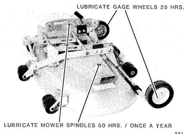
FIG. 22. Three Blade Mower Lubrication Fittings
