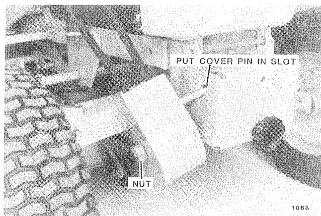
FIG. 13. Install Pulley Support Cover
