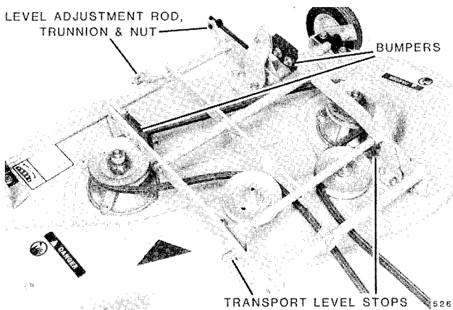
FIG. 17. 37 in. (94 cm) Mower Adjustments
