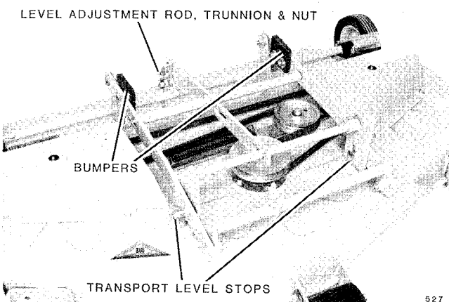
FIG. 18. 42 in. (107 cm) Rear Discharge Mower Adjustments
