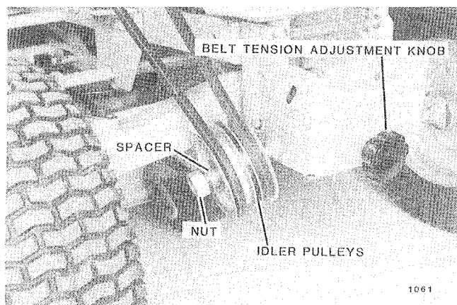
FIG. 11. 36, 42, 48 Inch Mower Front Idler Pulleys
