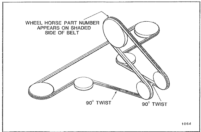
FIG. 8. 37 Inch Mower Drive Belt Routing
