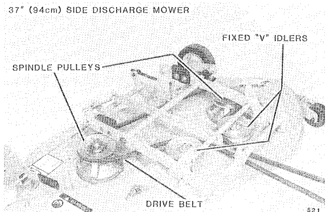
FIG. 9. 37 Inch Mower Drive Belt
