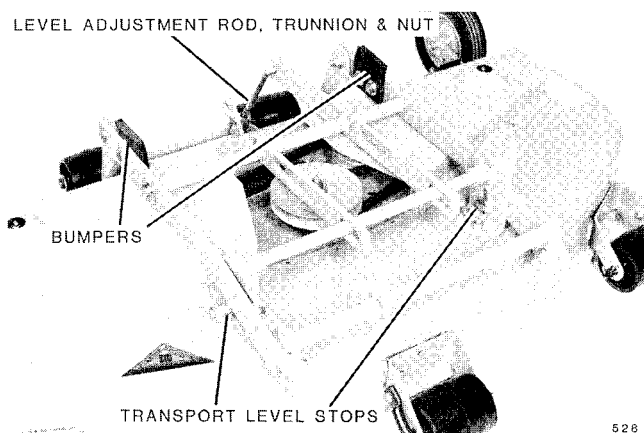
FIG. 20. 42 in. (107 cm) and 48 in. (122 cm) Side Discharge Mower Adjustments
