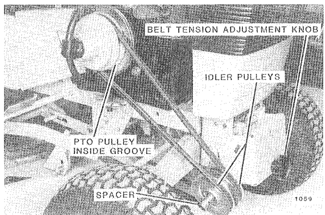
FIG. 10. 37 Inch Mower Front Idler Pulleys
