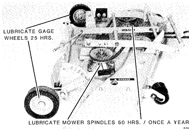
FIG. 21. Two Blade Mower Lubrication Fittings
