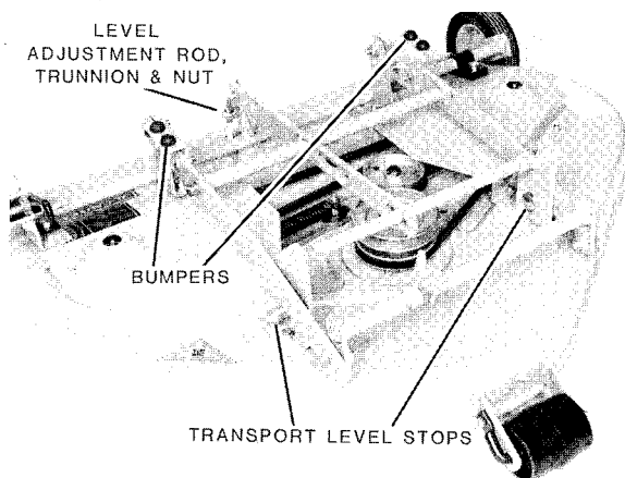
FIG. 16. 36 in. (92 cm) Mower Adjustments
