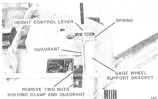
FIG. 1. Install Height Control Lever
