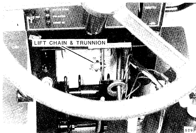
FIG. 19. Tractor Lift Bar Trunnion and Lift Rod Adjustment
