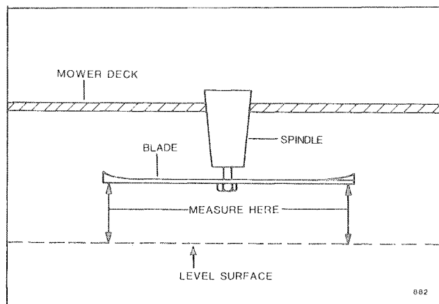
FIG. 14. Mower Level Measurement
