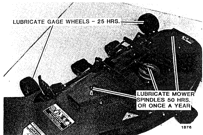
FIG. 19 Mower Lubrication Fittings
