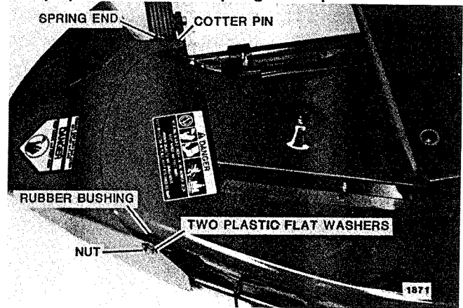
FIG. 2 Install Discharge Chute - Side Discharge Mower
