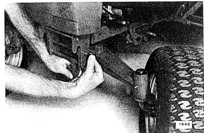
FIG. 8 Open Front Attach-A-Matic Hitch
