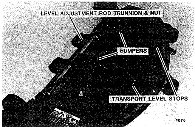
FIG. 17 48 in. (122 cm) Side Discharge Mower Adjustments
