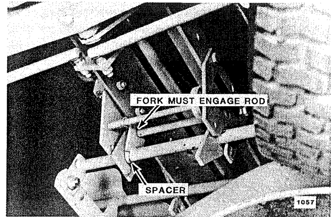
FIG. 6 Align Fork with Shaft
