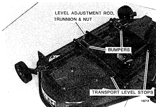
FIG. 15 42 in. (107 cm) Rear Discharge Mower Adjustments
