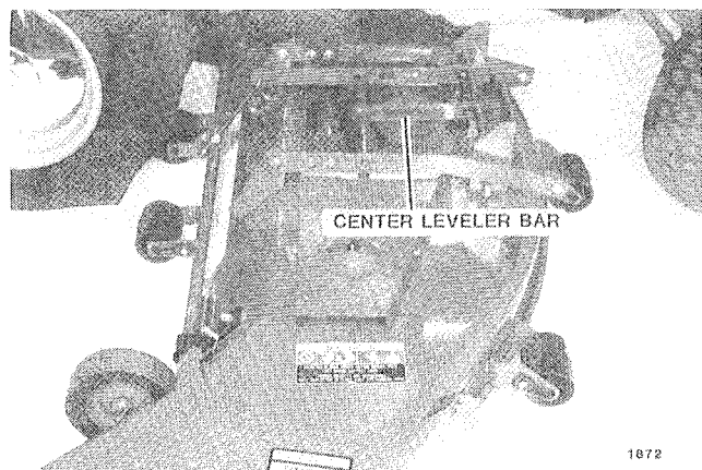
FIG. 3. Position Mower to Right of Tract
