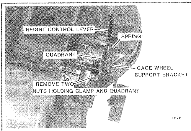
FIG. 1 Install Height Control Lever - 42" Rear Discharge Mower
