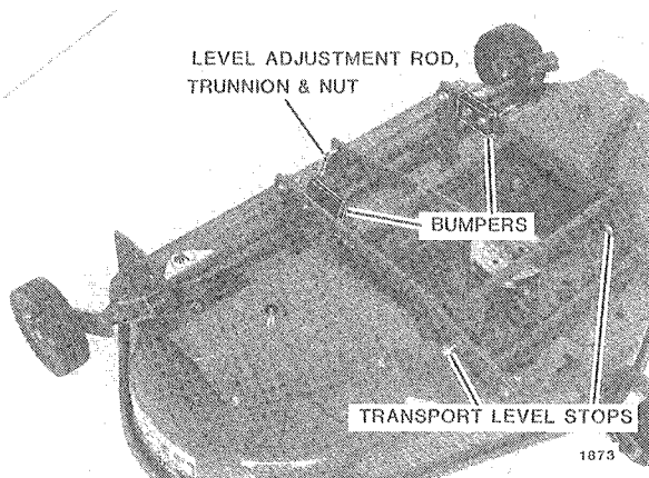
FIG. 15 42 in. (107 cm) Rear Discharge Mower Adjustments
