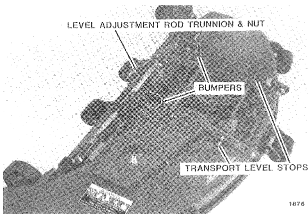
FIG. 17 48 in. (122 cm) Side Discharge Mower Adjustments
