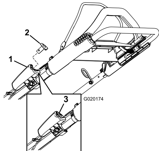
Figure 12 Electric start
