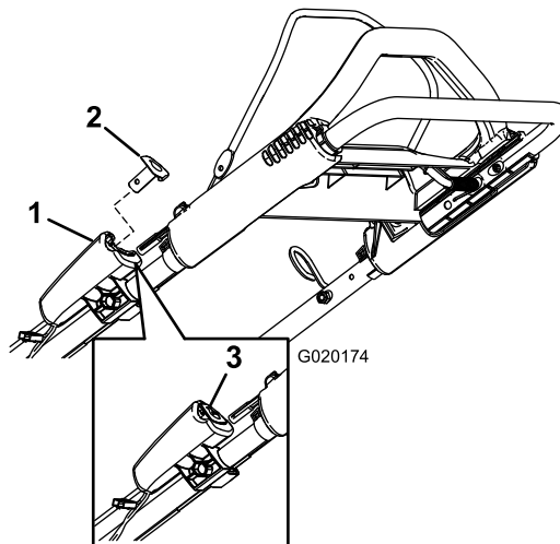
Figure 12 Electric start
