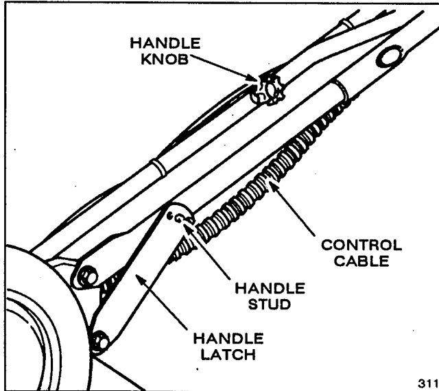
Self-propelled model
