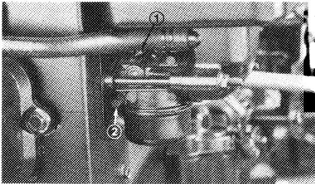
Figure 20 1. Idle speed screw 2. Idle fuel screw
