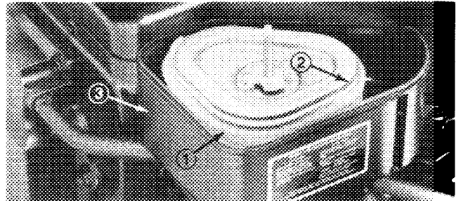
Figure 15 1. Foam element 2. Paper element 3. Air cleaner body
