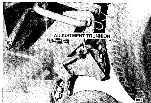
FIG. 8 Side-To-Side Adjustment
