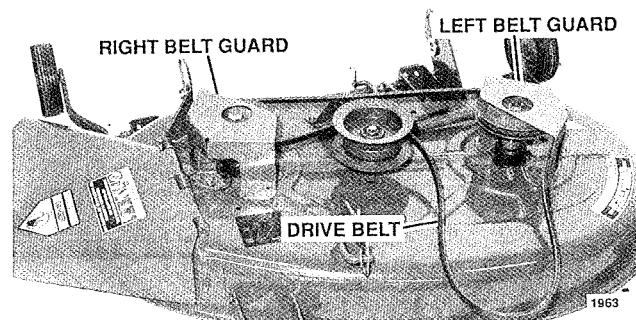
FIG. 12. Drive Belt Routing
