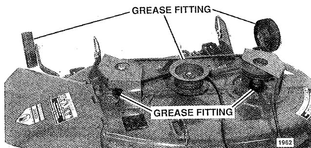
FIG. 11. Grease Fittings
