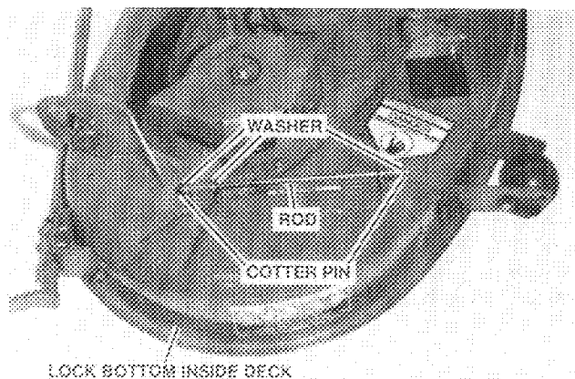
FIG. 10 Discharge Cover
