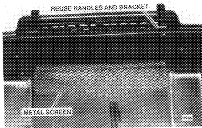
FIG. 3 Install Metal Screen
