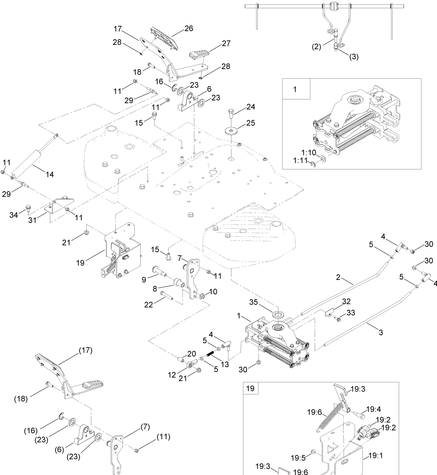
FOOT PEDAL ASSEMBLY
