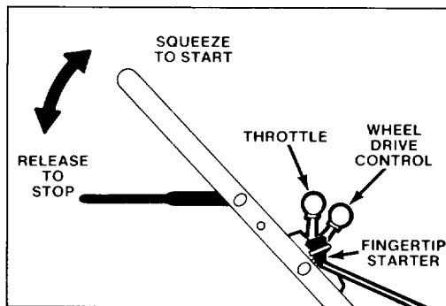
Self-Propelled Model 16775
