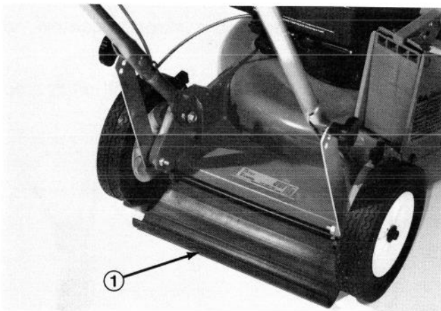
Figure 17 1. Rear shield
