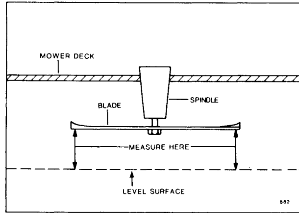
FIG. 10. Mower Level Measurement
