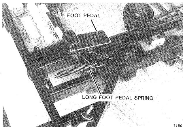
FIG. 5. Long Foot Pedal Spring
