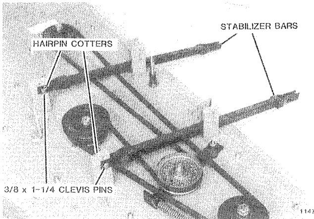
FIG. 2. Install Stabilizer Bars
