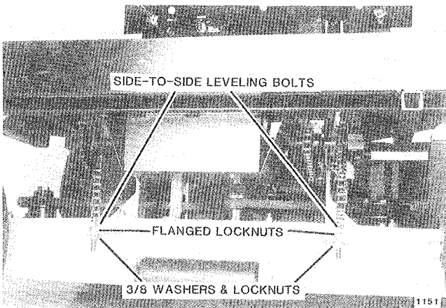
FIG. 9. Side-To-Side Level Adjustment
