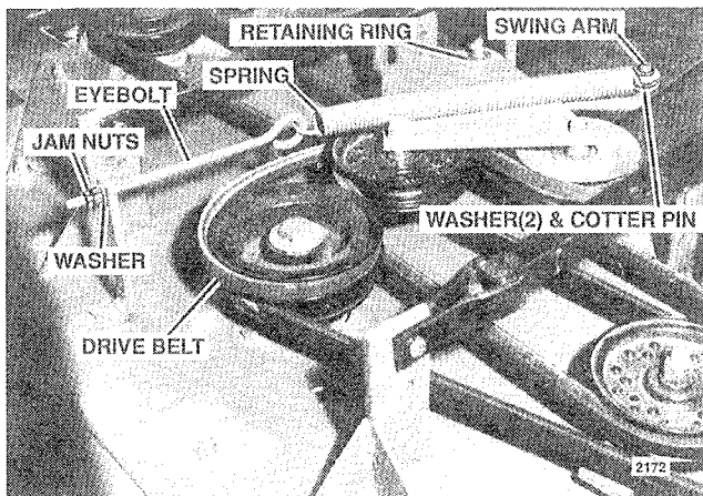
FIG. 3. Install Mower Belt Tensioning Swing Arm, Spring and Drive Belt
