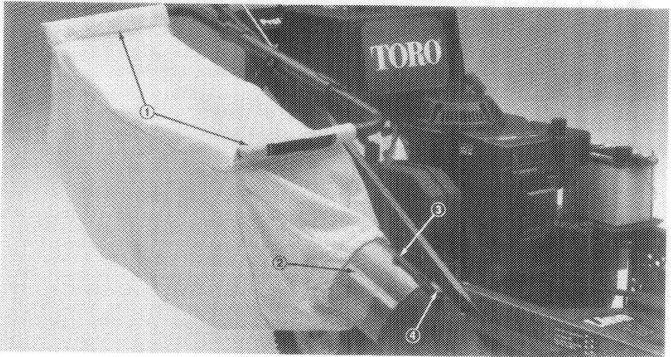
Figure 9 1. Bag Seams 2. Duct 3. Duct Retainer 4. Chute Knob
