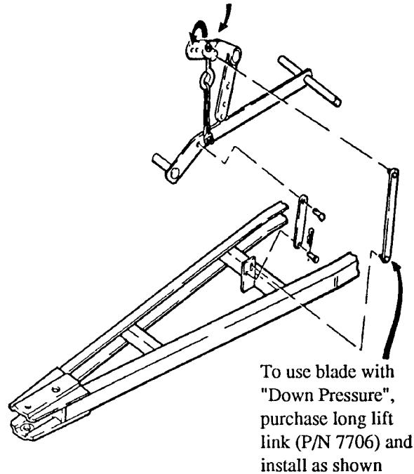
FIG. 19 Linkage Connections
