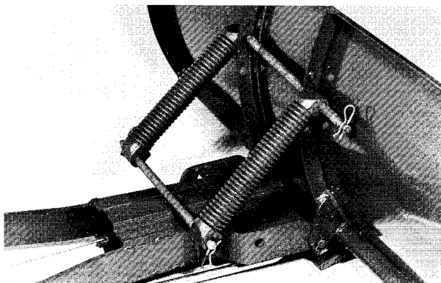
FIG. 12 Attach Trip Springs to Blade
