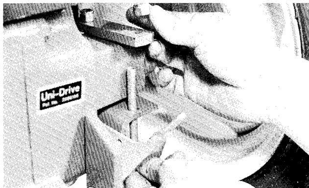
FIG. 8 Install Two 3/8-16 x 3 3/4 Carriage Bolts & Nuts
