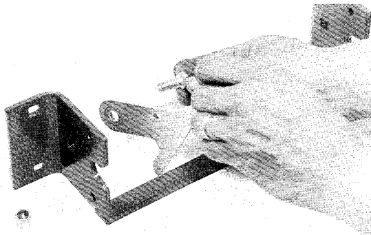
FIG. 5 Attach Latching Plates to Mounting Bracket
