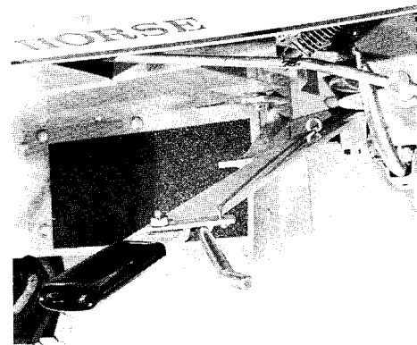
FIG. 18 Attach Release Lever to Index Handle
