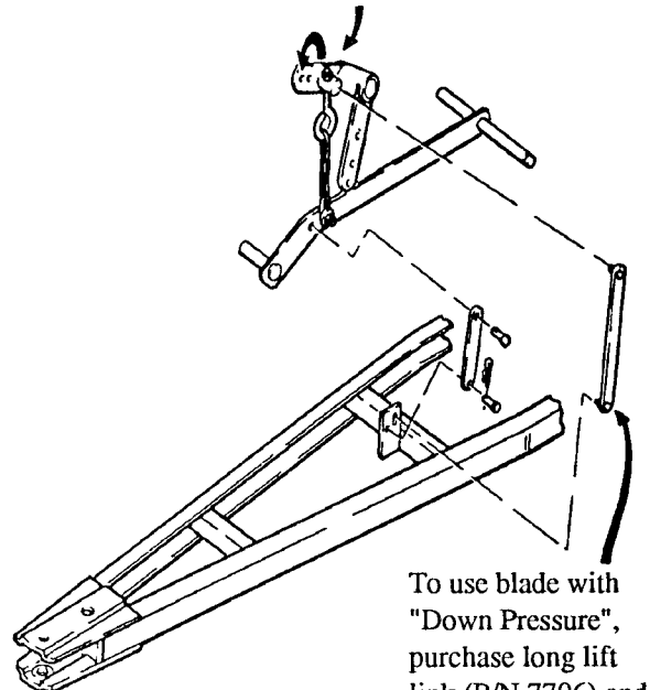
FIG. 19 Linkage Connections
