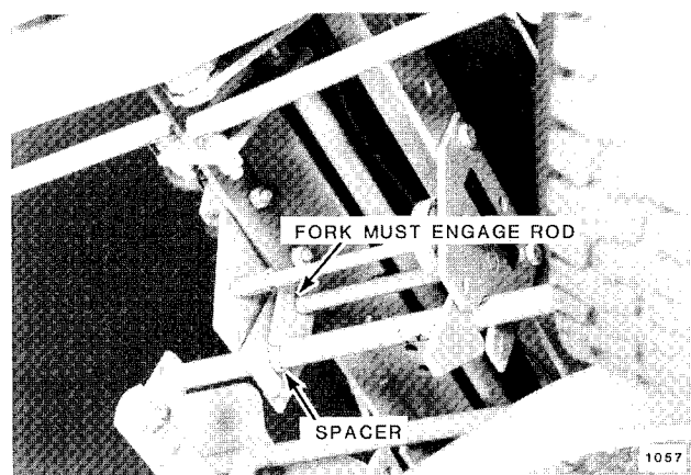
FIG. 4. Align Fork with Shaft
