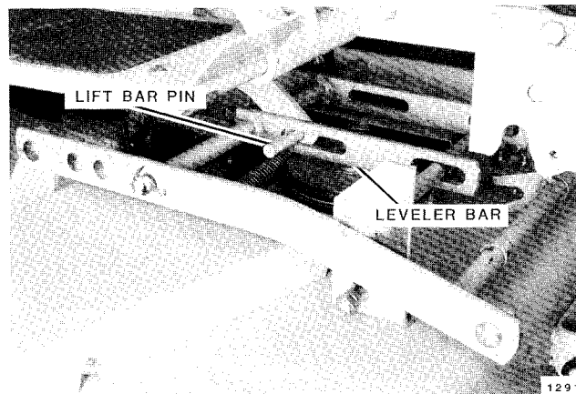
FIG. 2. Align Pin with Slot
