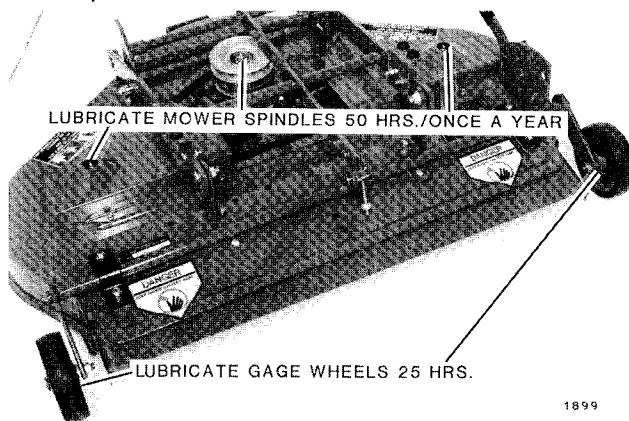
FIG. 14. Mower Lubrication Fittings
