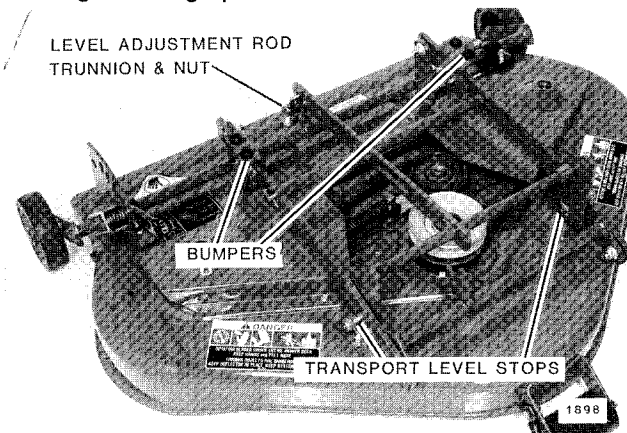
FIG. 12. Mower Adjustments
