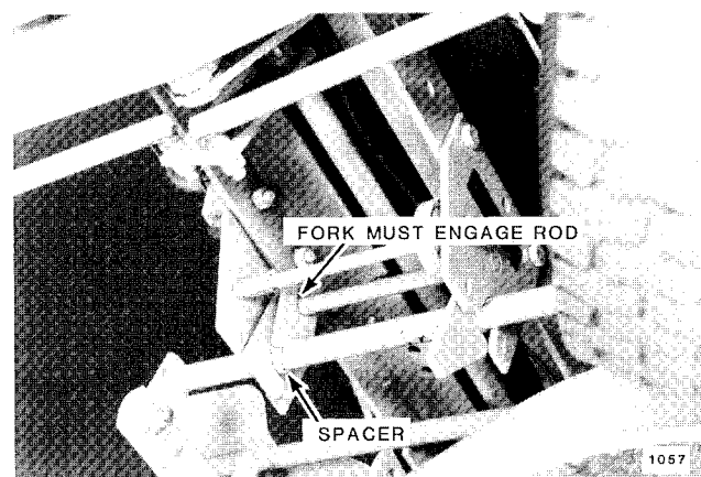
FIG. 4. Align Fork with Shaft
