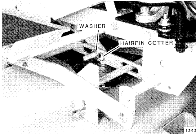
FIG. 5. Secure Mower to Tractor Lift Bar Pin
