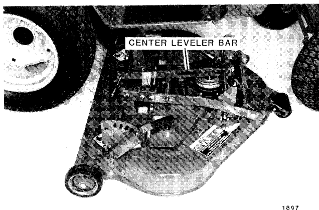
FIG. 1. Position Mower to Right of Tractor
