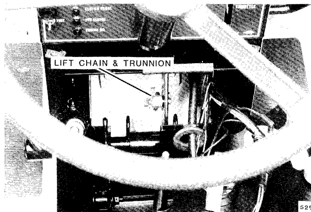
FIG. 13. Tractor Lift Bar Trunnion and Lift Rod Adjustment
