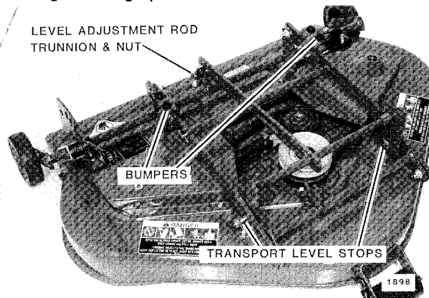
FIG. 12. Mower Adjustments
