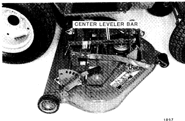
FIG. 1. Position Mower to Right of Tractor
