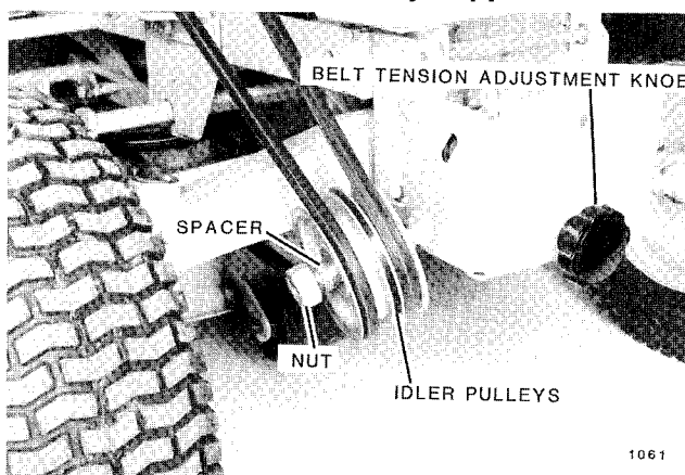
FIG. 8. Mower Front Idler Pulleys
