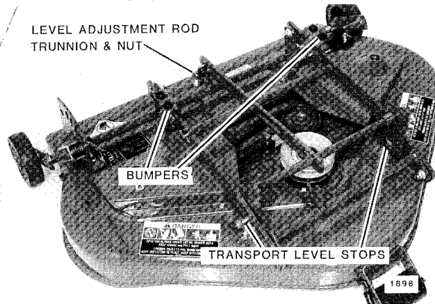
FIG. 12. Mower Adjustments
