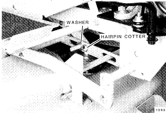
FIG. 5. Secure Mower to Tractor Lift Bar Pin
