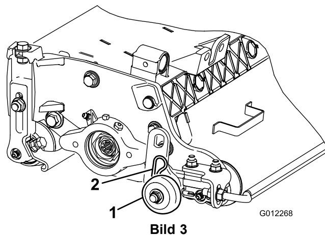
1. Transportrollen
