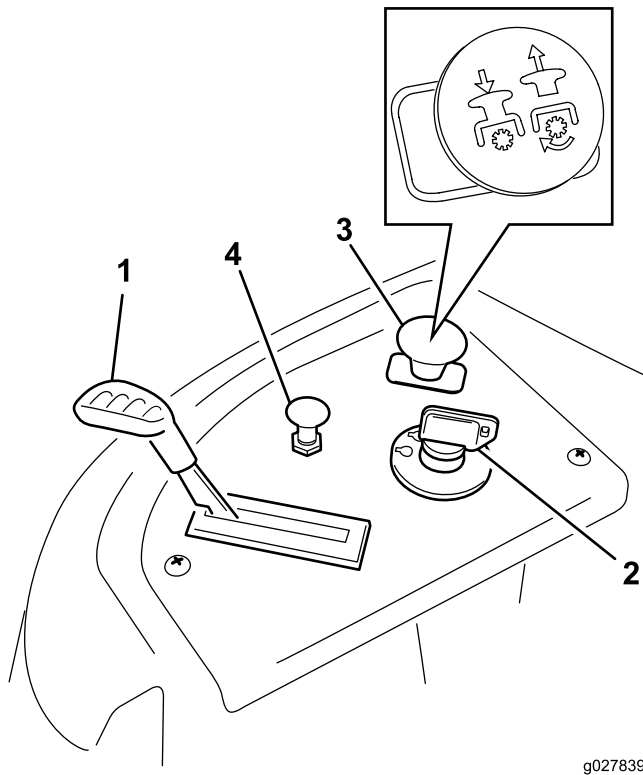
Figure 6 Control Panel
