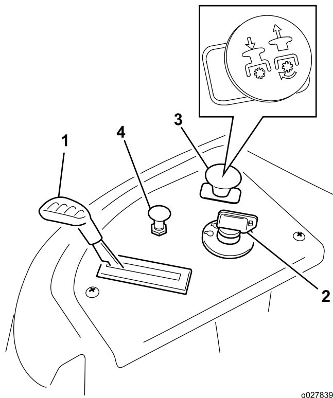
Figur 6 Kontrollpanel
