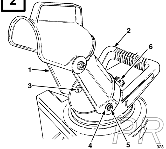
1. Discharge chute 2. Chute handle 3. Hex bolt 4. Washer 5. Locknut 6. Knob
