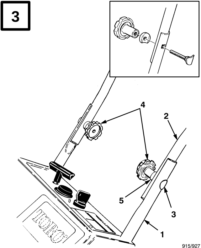
1. Lower 2. Upper handle 3. Oval head bolt 4. Knob 5. Curved washers
